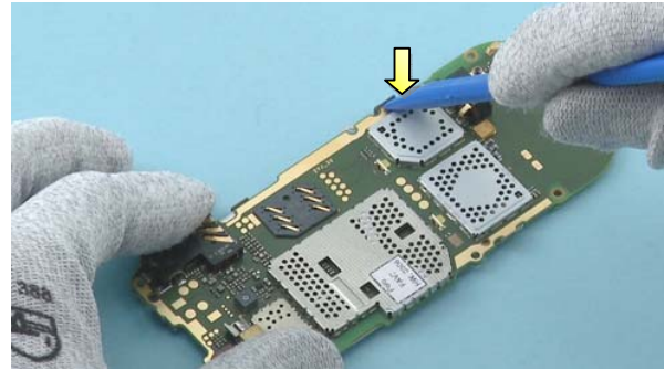
20) Release the second clip on the left side of the UI SHIELDING using the SS-93.
