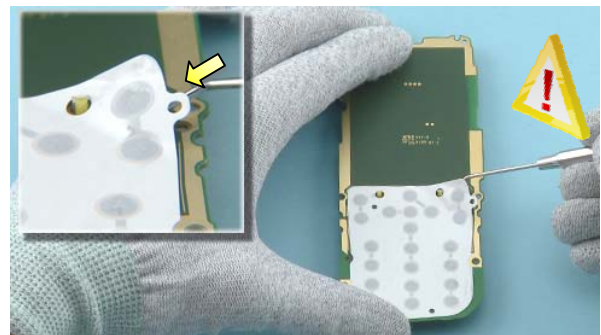
24) Use the dental tool to lift an edge of the DOME SHEET. Be careful not to damage the DOME SHEET or the PWB!
