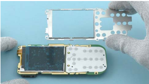
21) Remove the UI SHIELDING.
