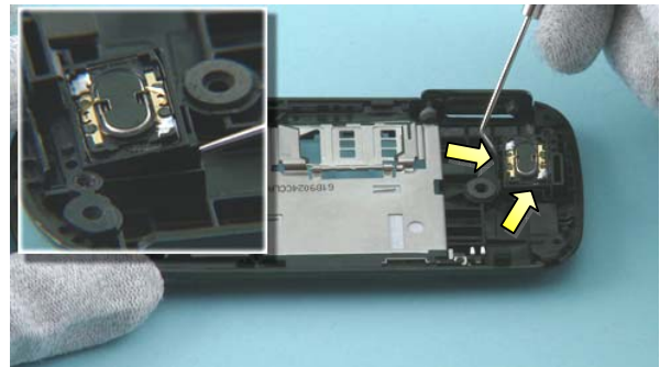
16) Use the dental tool to lever out the EARPIECE MODULE.
