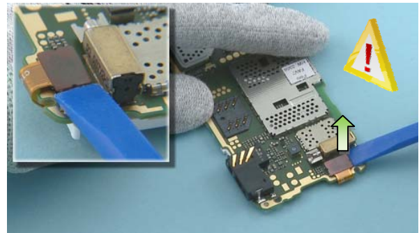
22) Carefully release the LCD connector using the SS-93. Be careful not to damage the connector or any other components nearby!
