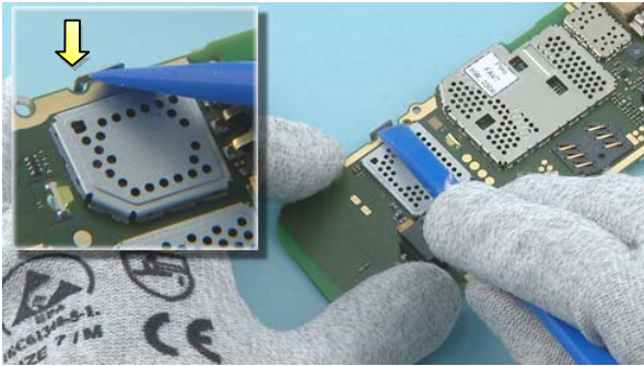
19) On the right side of the UI SHIELDING, release the first clip using the SS-93.
